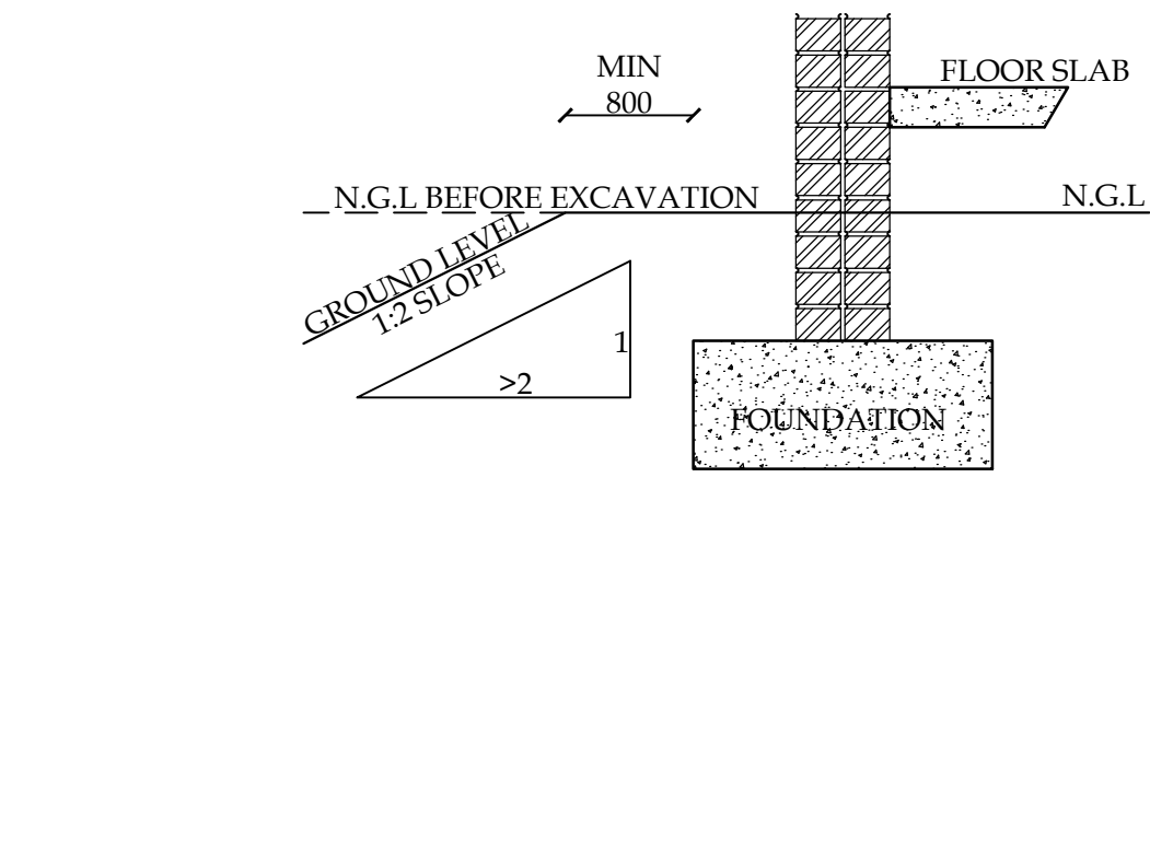
PERMANENT EXCAVATION DETAIL SCALE 1:20
