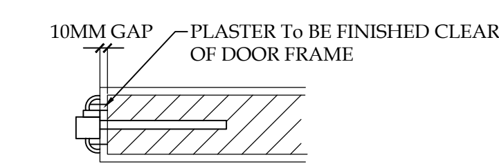
SOLID TIMBER FRAME DETAIL SCALE N.T.S
