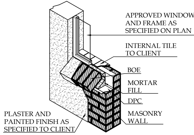
BOE WINDOW CILL DETAIL SCALE 1:20
