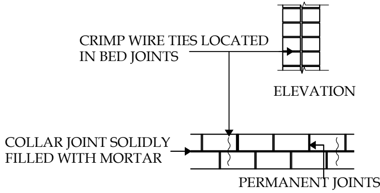
COLLAR JOINTED WALL DETAIL
