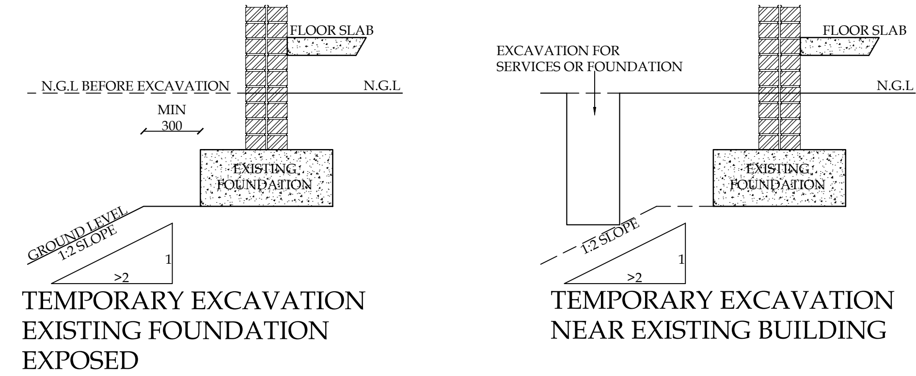
TEMPORARY EXCAVATION DETAIL SCALE 1:20
